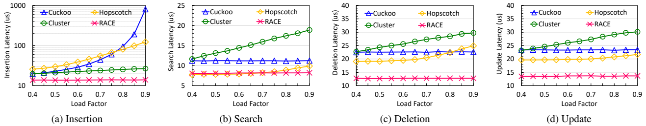
Figure 10: Average latencies of different requests when hash tables are in different load factors.
