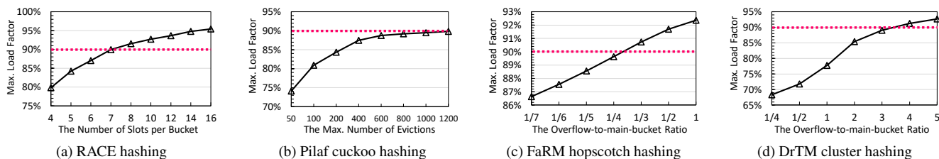
Figure 9: Maximum load factors of different hash tables. (In FaRM hopscotch hashing and DrTM cluster hashing, overflow buckets indicate the buckets linked in conflicting lists. The load factor indicates the ratio of the number of occupied slots to that of all slots in both overflow and main buckets. The overflow-to-main-bucket ratio means the ratio of the number of overflow buckets to that of main buckets.)
