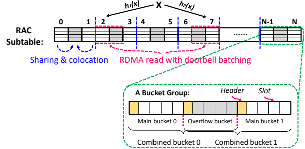
Figure 4: The RAC hash subtable structure (4-way associativity as an example).
